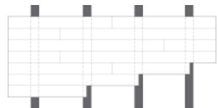
Fig.2. Butt joints for end matched boards.
